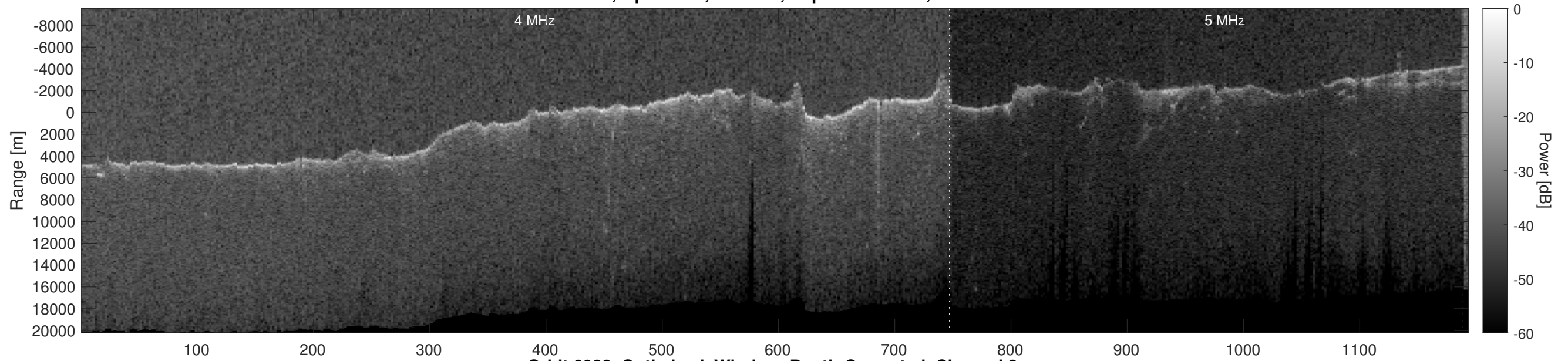
Orbit 6988, Optimized, Window, Depth-Corrected, Channel 2
