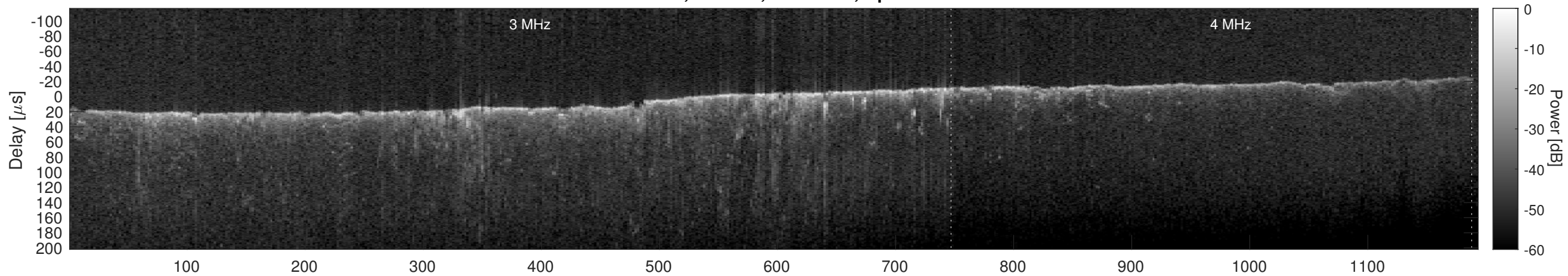
Orbit 6990, Cluttergram
