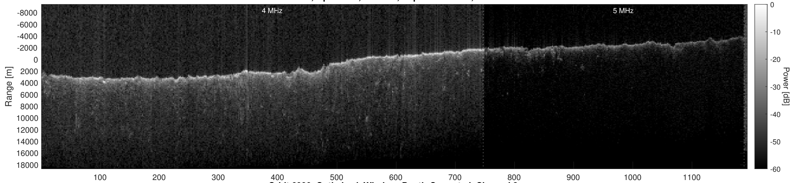
Orbit 6990, Optimized, Window, Depth-Corrected, Channel 2
