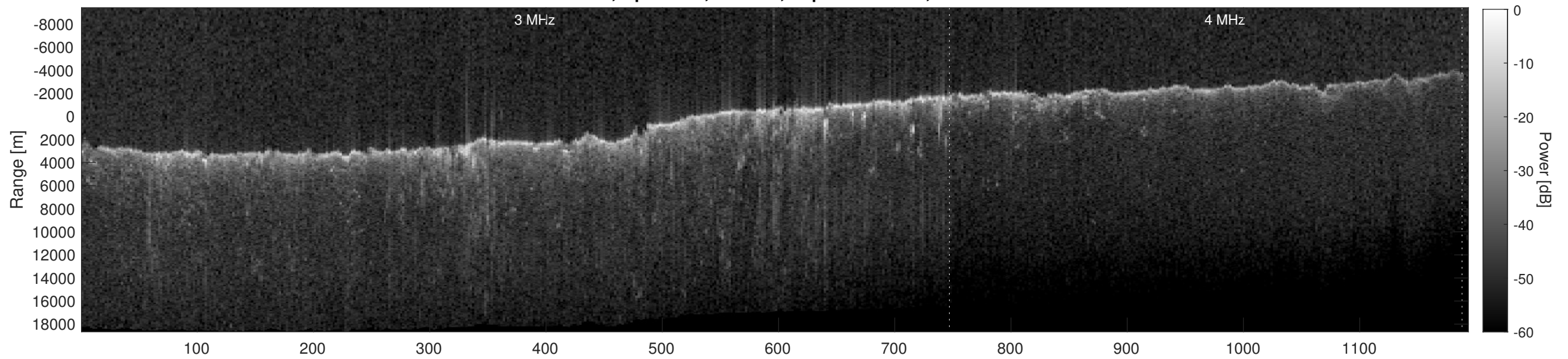
Orbit 6990, Depth-Corrected Cluttergram
