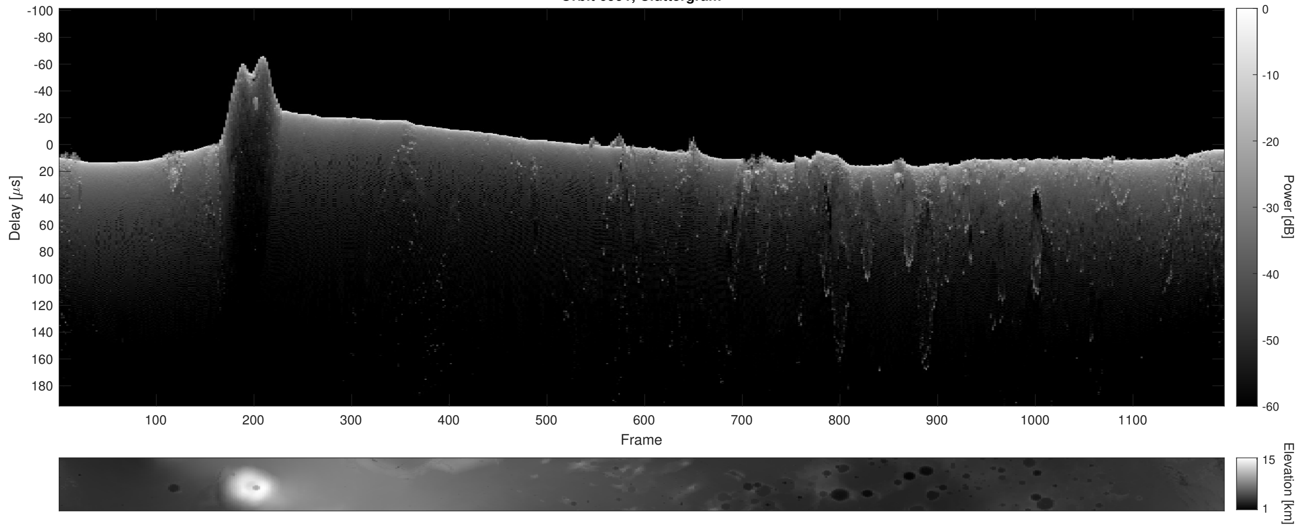
Orbit 6991, Cluttergram
