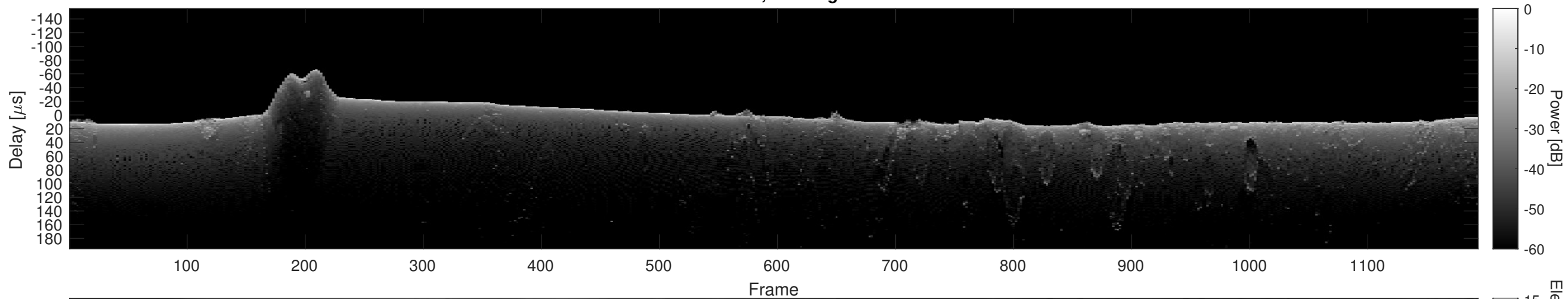
Orbit 6991, Cluttergram
