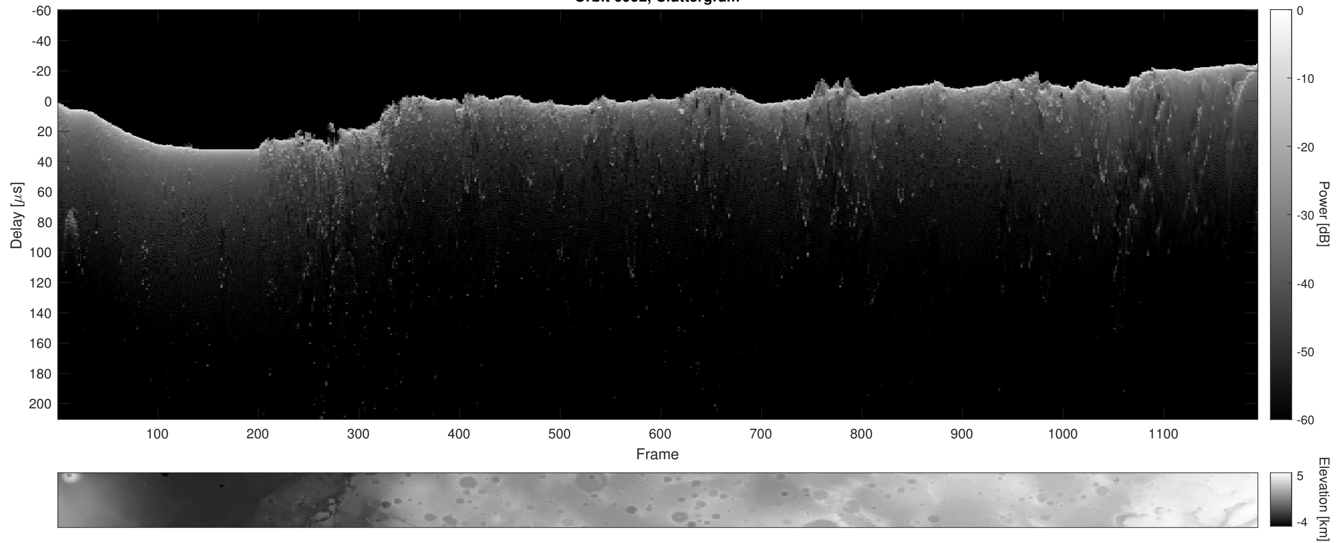
Orbit 6992, Cluttergram
