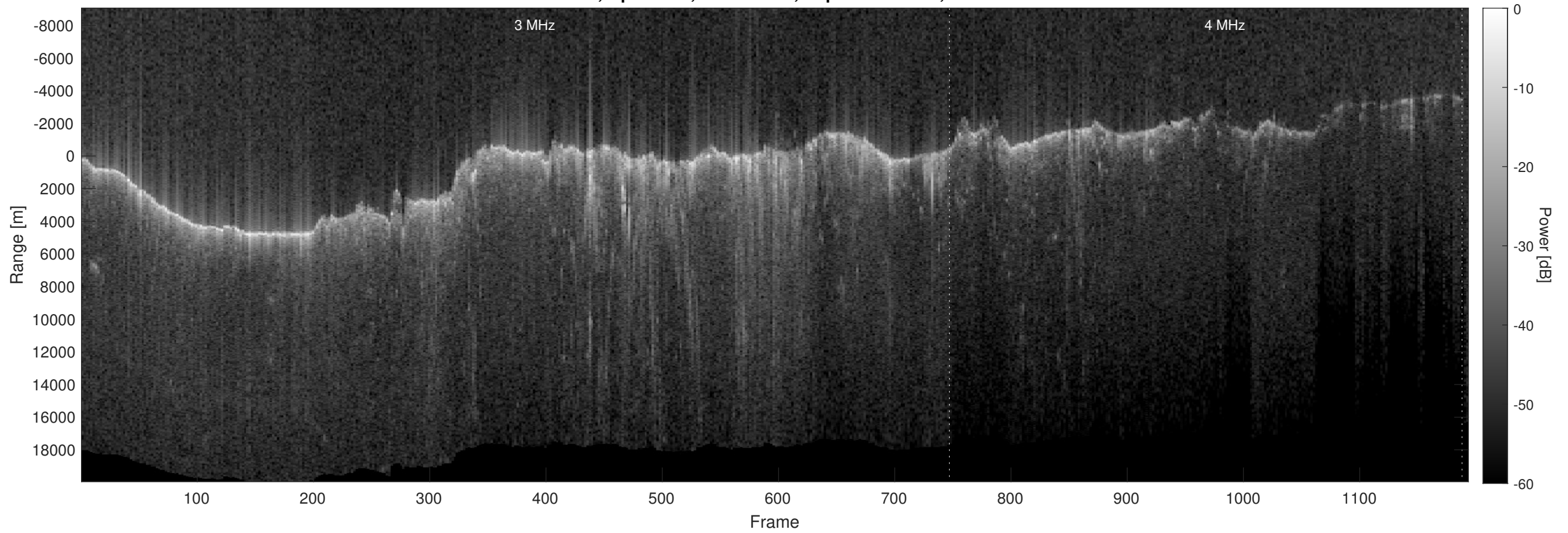
Orbit 6992, Optimized, No Window, Depth-Corrected, Channel 2
