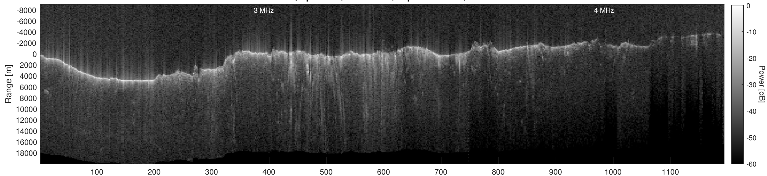
Orbit 6992, Depth-Corrected Cluttergram
