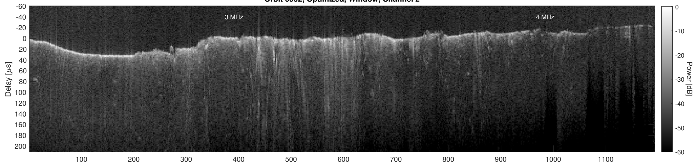
Orbit 6992, Cluttergram
