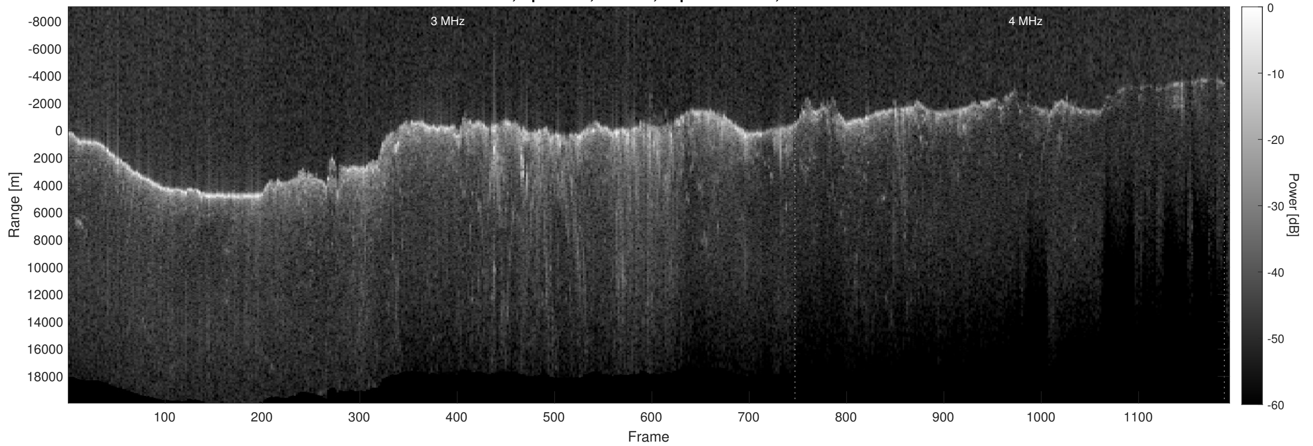
Orbit 6992, Optimized, Window, Depth-Corrected, Channel 2
