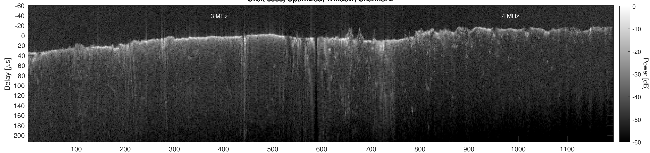
Orbit 6996, Cluttergram
