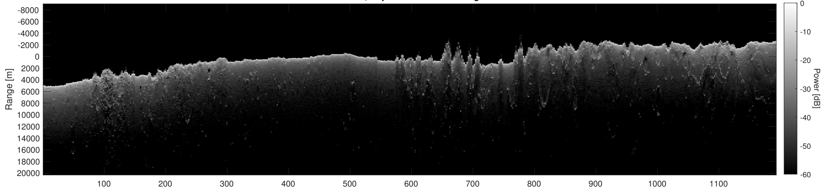
Orbit 6996, Depth-Corrected Cluttergram
