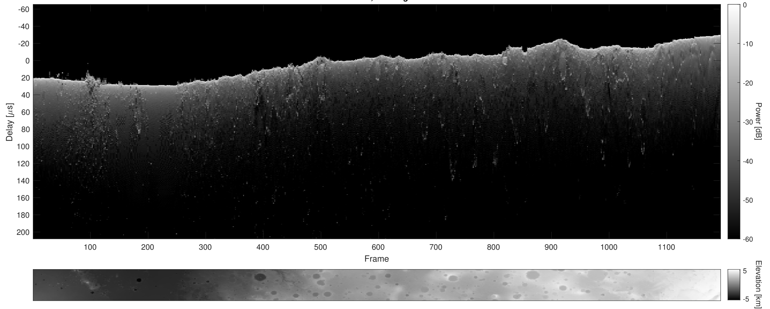
Orbit 6999, Cluttergram
