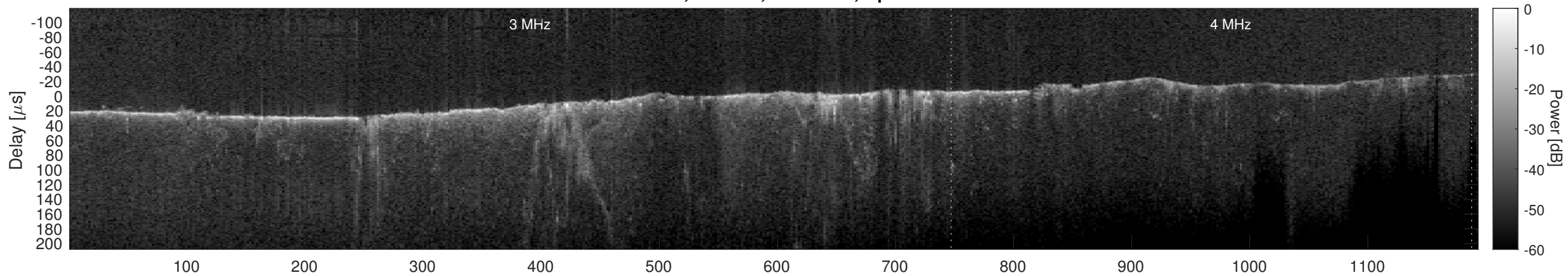
Orbit 6999, Cluttergram
