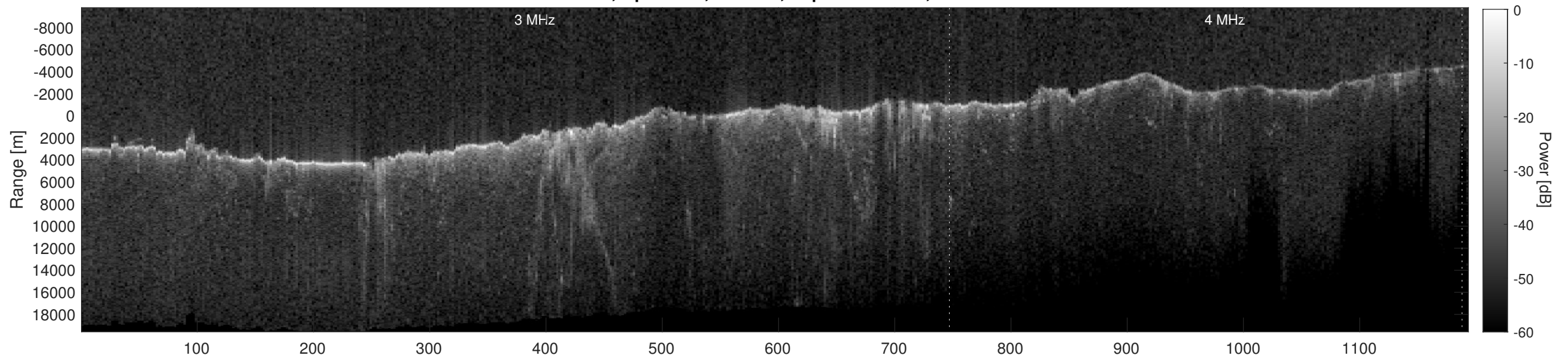
Orbit 6999, Depth-Corrected Cluttergram
