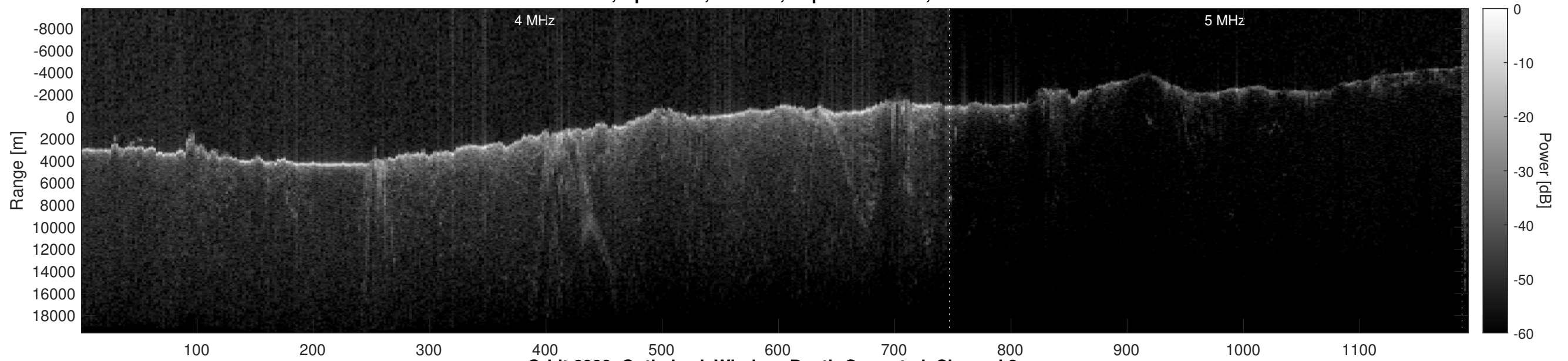
Orbit 6999, Optimized, Window, Depth-Corrected, Channel 2
