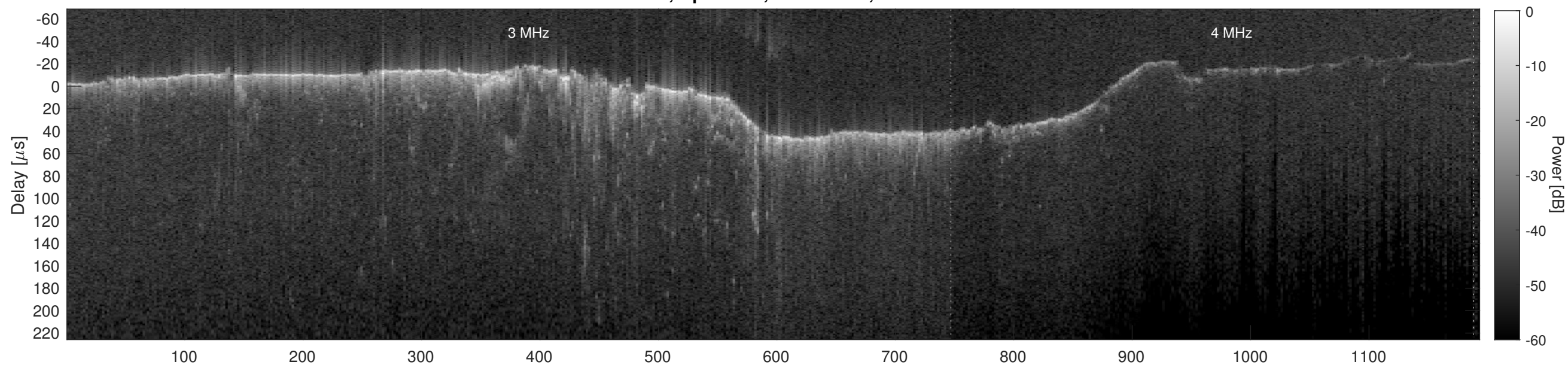
Orbit 7000, Cluttergram
