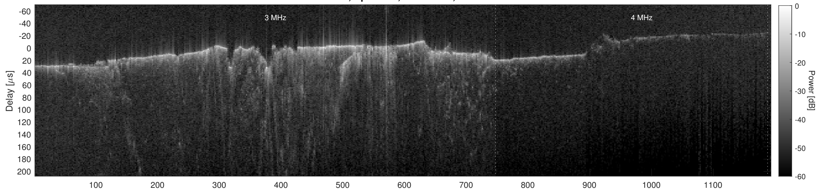
Orbit 7001, Cluttergram
