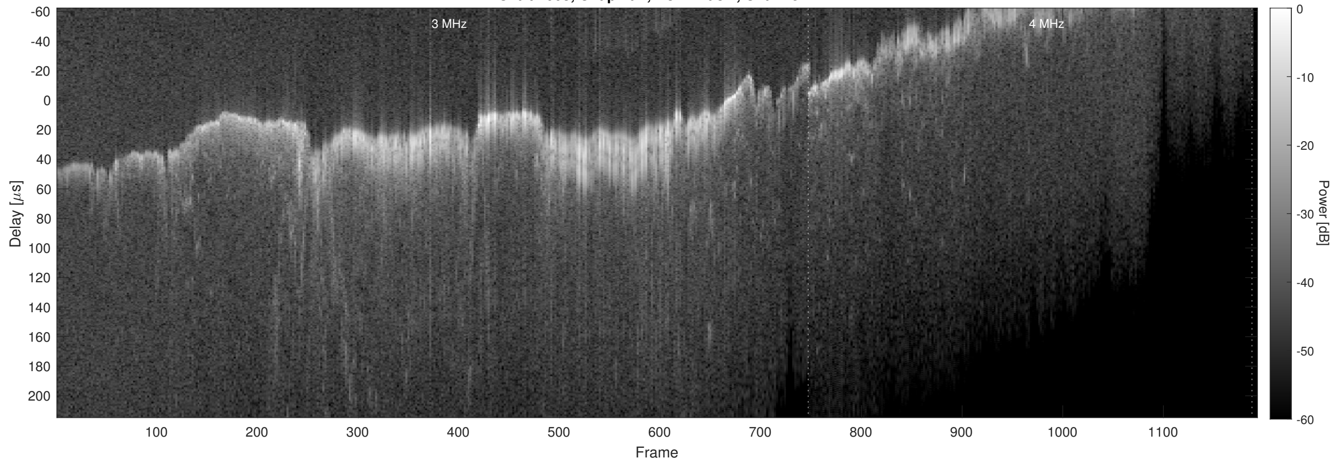
Orbit 7003, Chapman, No Window, Channel 2
