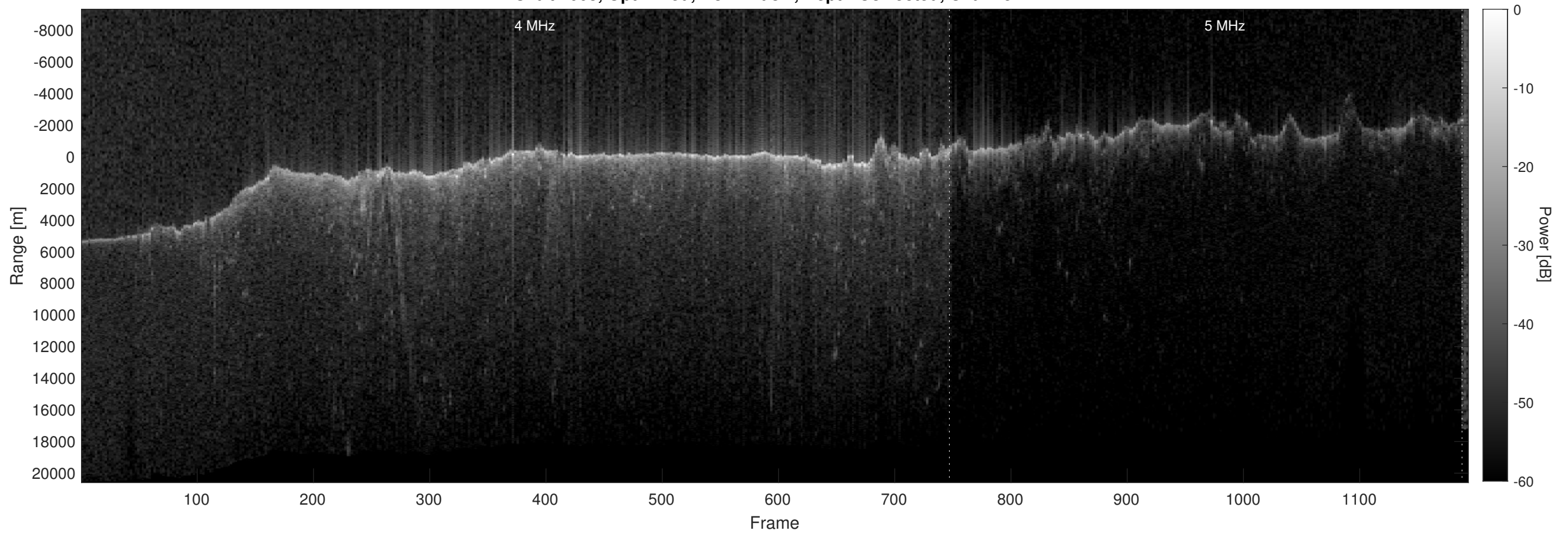
Orbit 7003, Optimized, No Window, Depth-Corrected, Channel 2
