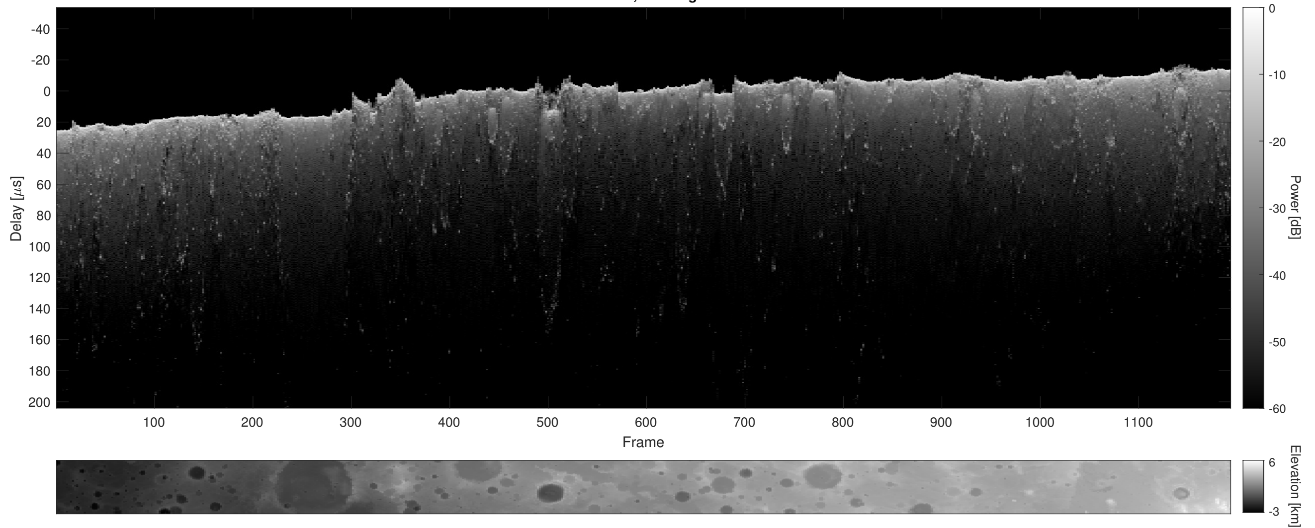
Orbit 7004, Cluttergram
