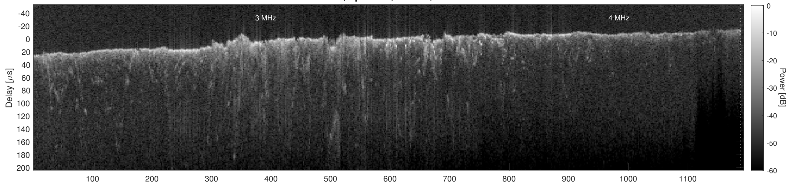
Orbit 7004, Cluttergram
