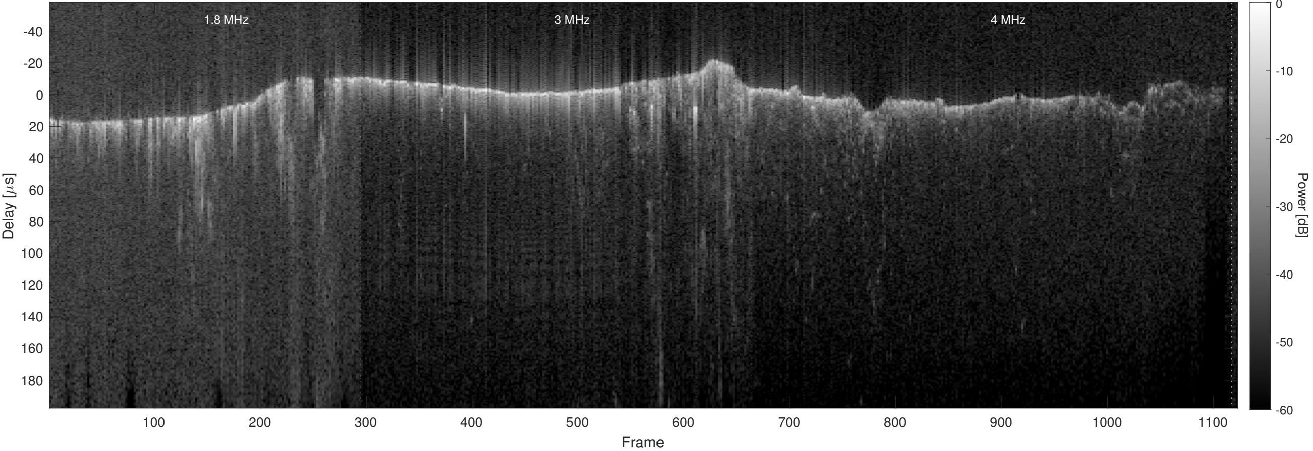
Orbit 7005, Optimized, No Window, Channel 2
