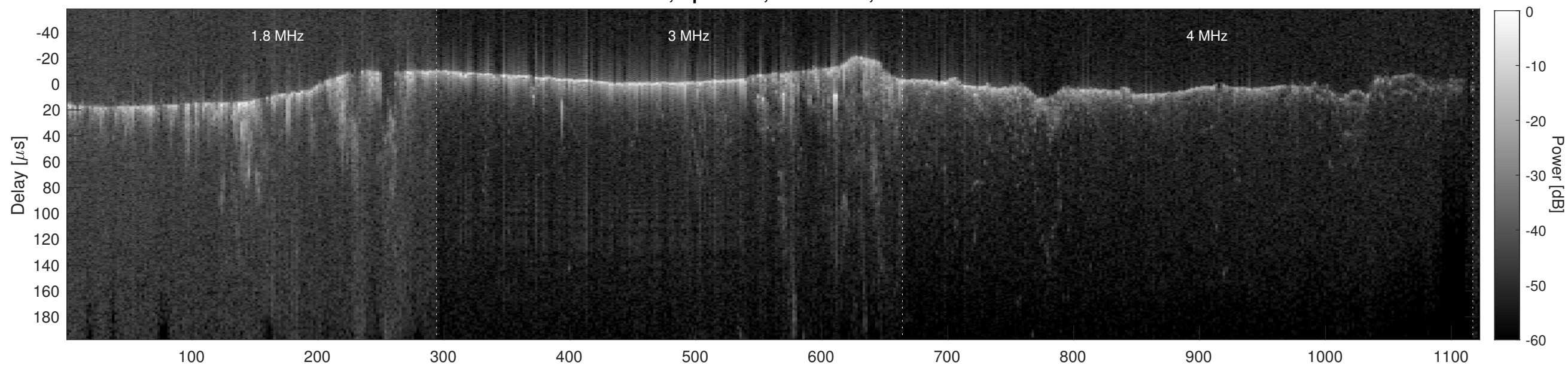
Orbit 7005, Cluttergram
