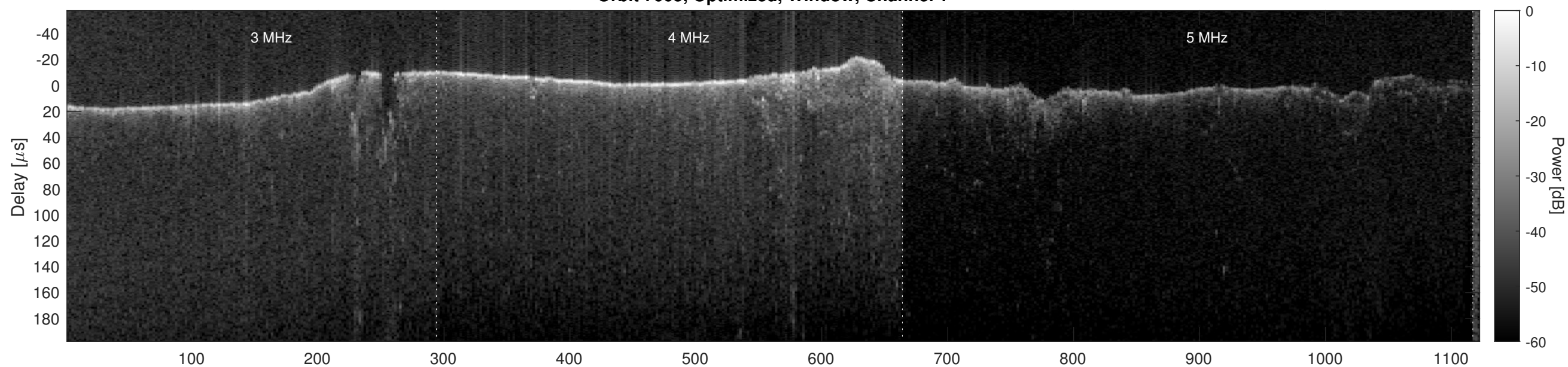
Orbit 7005, Optimized, Window, Channel 2
