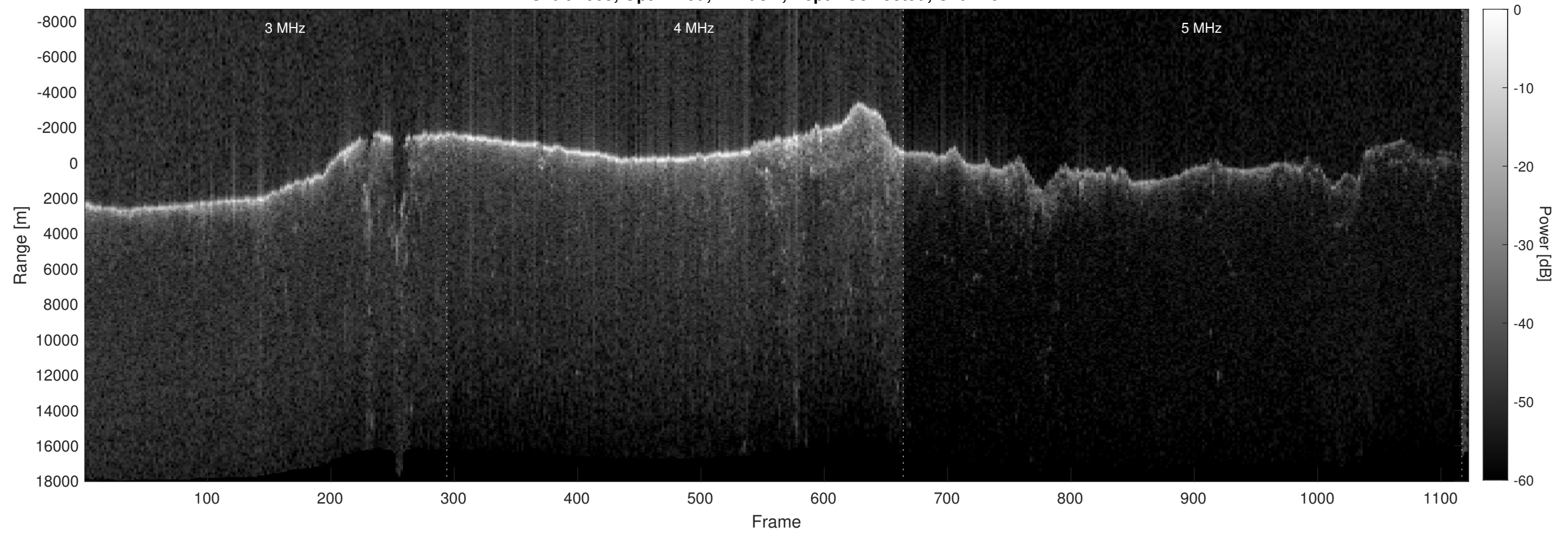
Orbit 7005, Optimized, Window, Depth-Corrected, Channel 2
