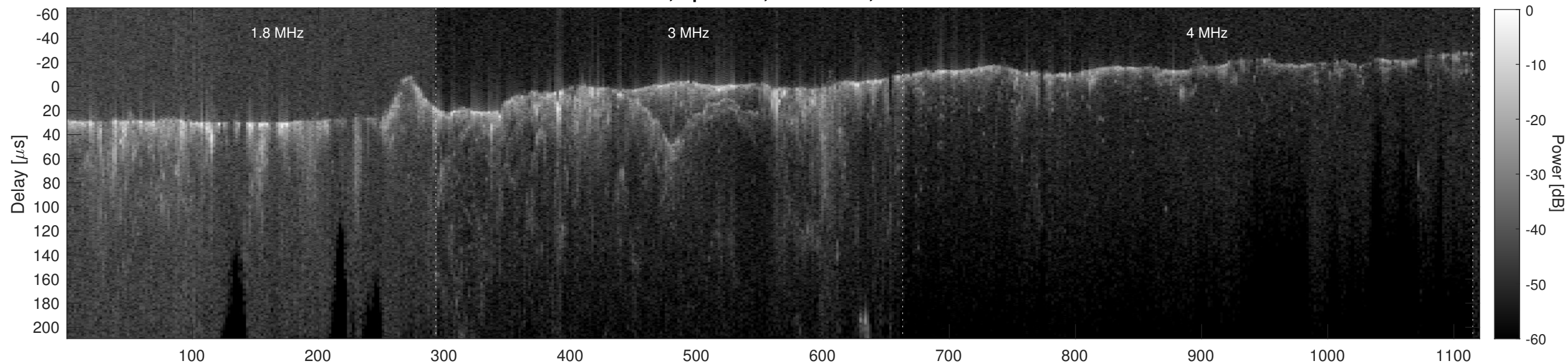
Orbit 7006, Cluttergram
