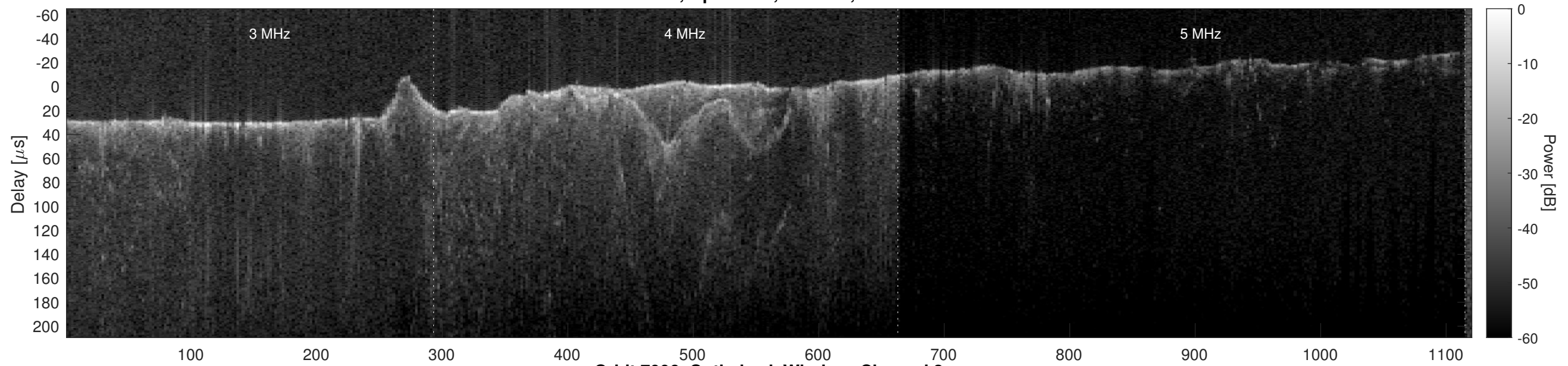
Orbit 7006, Optimized, Window, Channel 2
