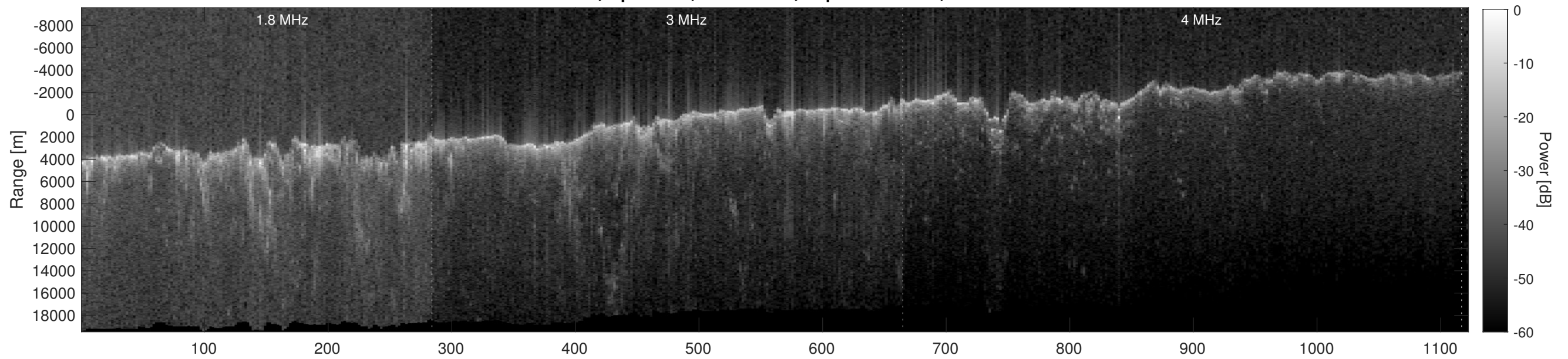
Orbit 7008, Depth-Corrected Cluttergram
