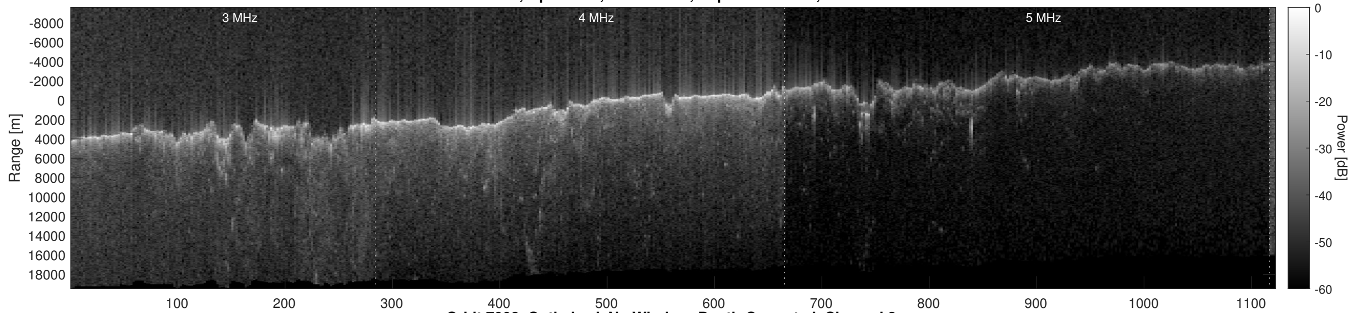
Orbit 7008, Optimized, No Window, Depth-Corrected, Channel 2
