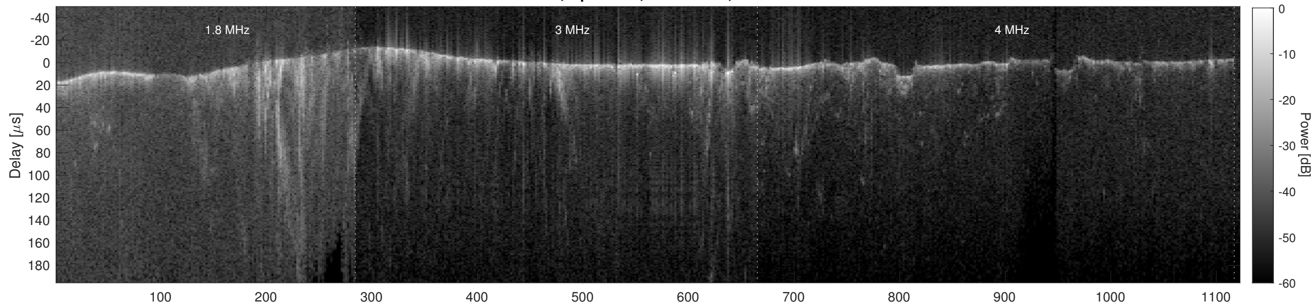
Orbit 7009, Cluttergram
