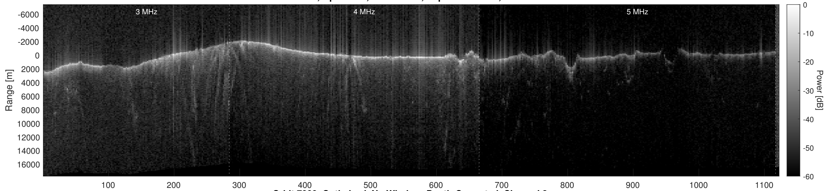
Orbit 7009, Optimized, No Window, Depth-Corrected, Channel 2
