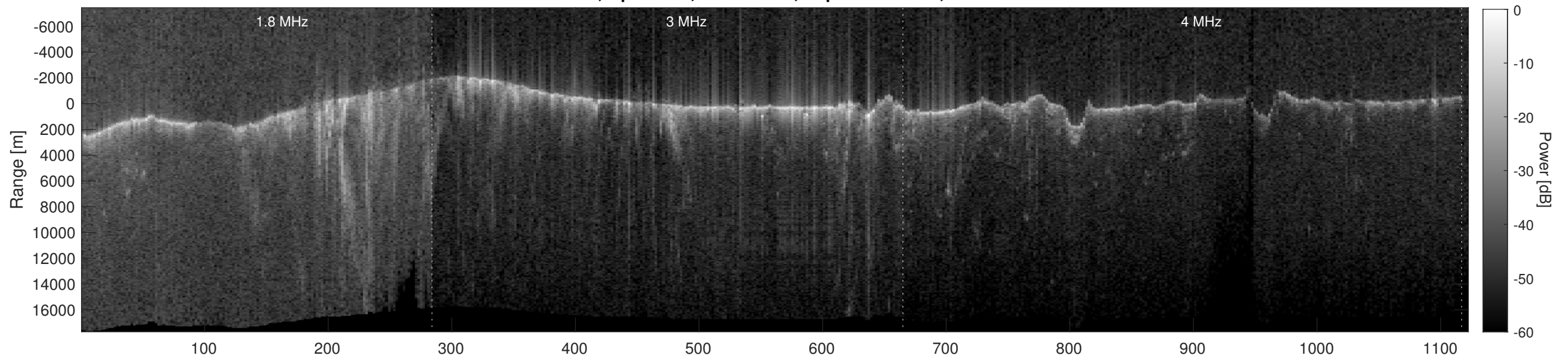
Orbit 7009, Depth-Corrected Cluttergram
