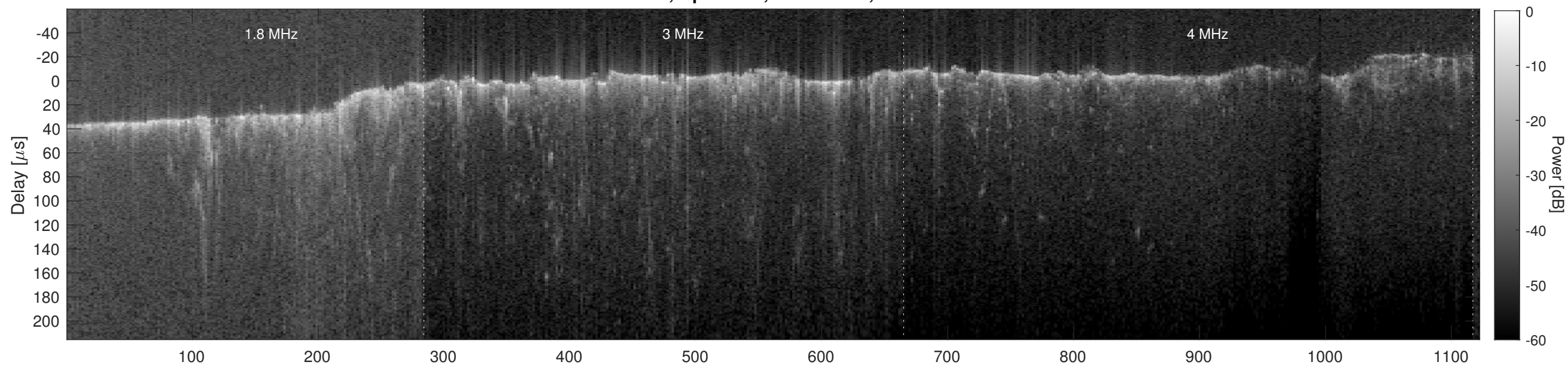
Orbit 7010, Cluttergram
