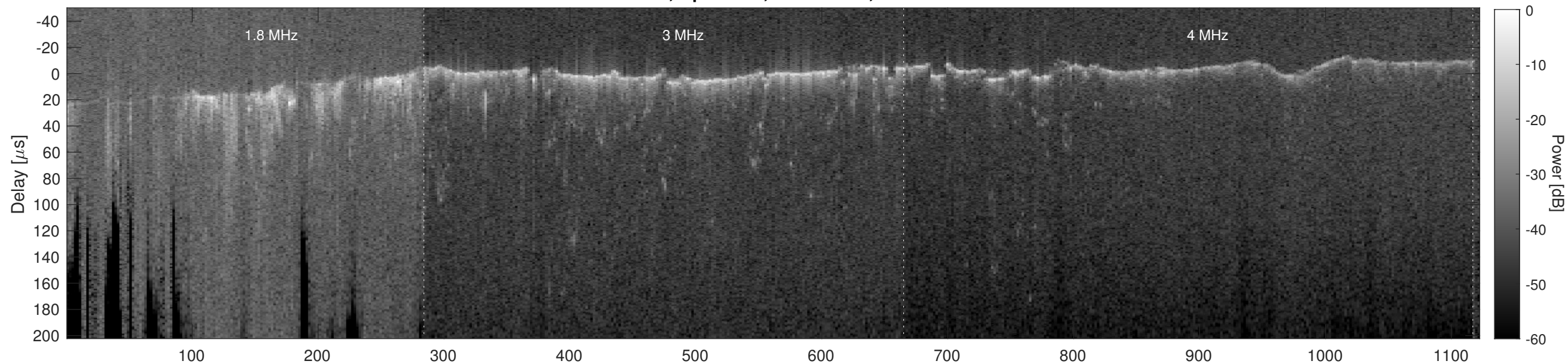
Orbit 7011, Cluttergram
