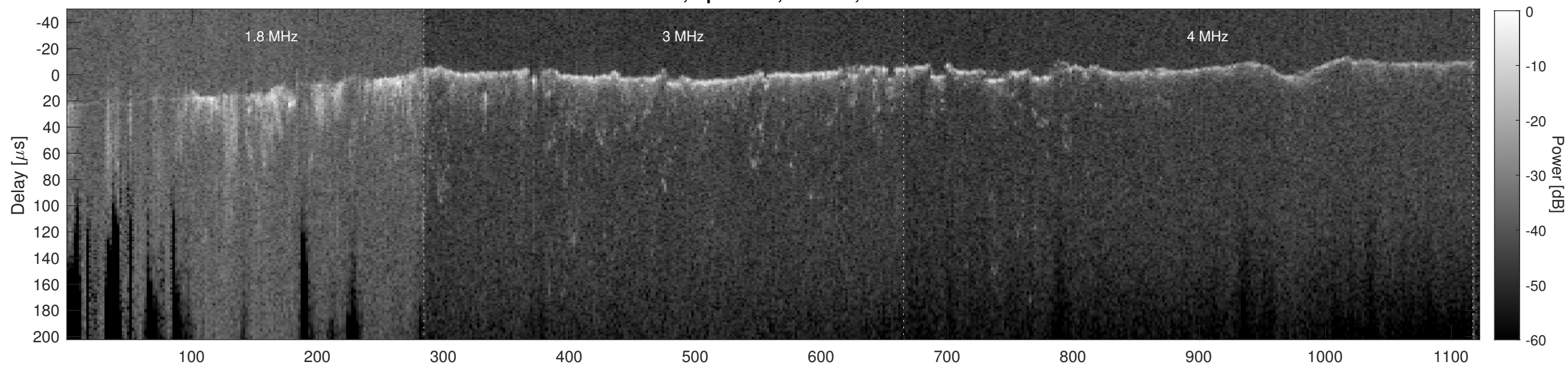
Orbit 7011, Cluttergram
