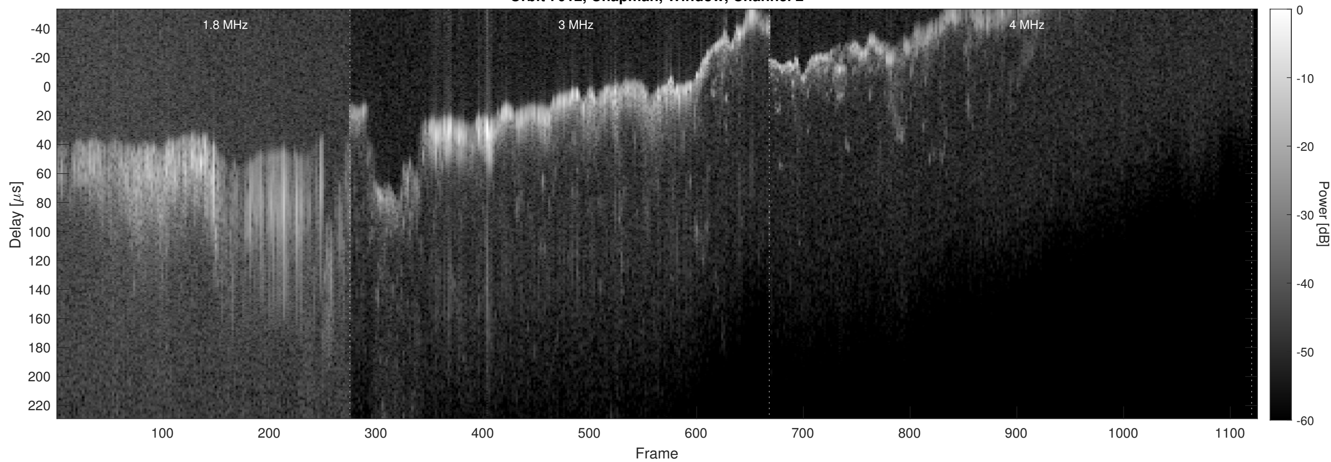
Orbit 7012, Chapman, Window, Channel 2
