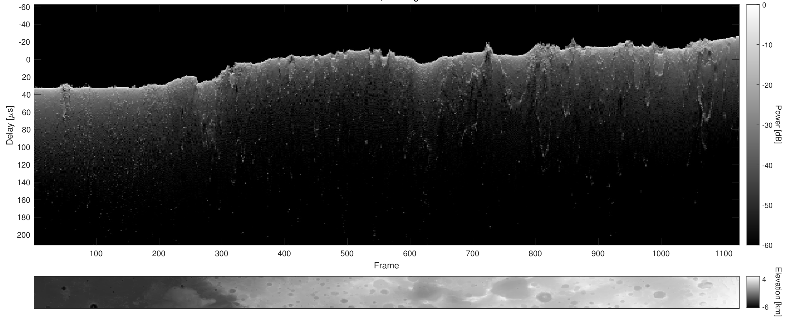
Orbit 7013, Cluttergram
