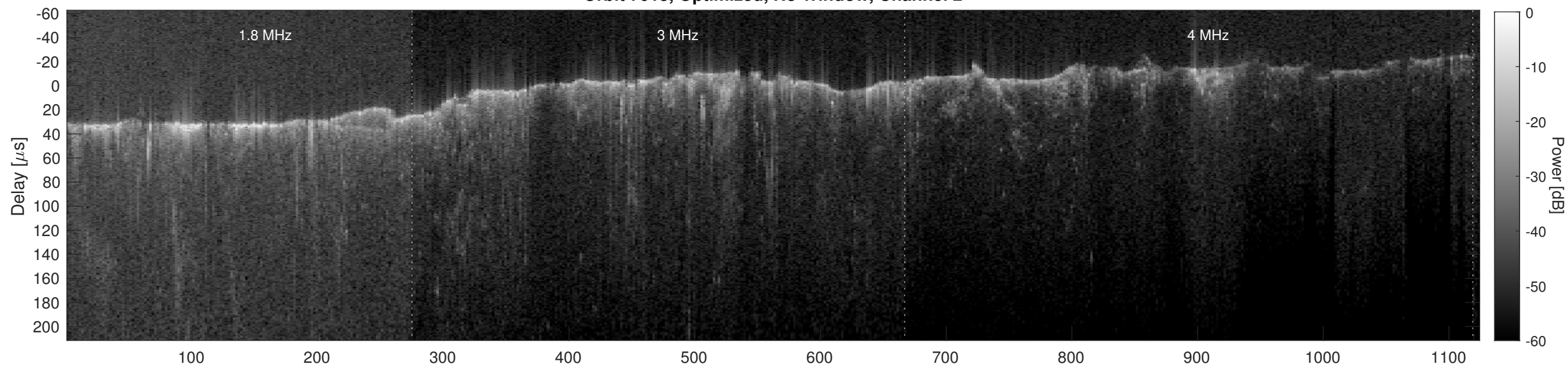
Orbit 7013, Cluttergram
