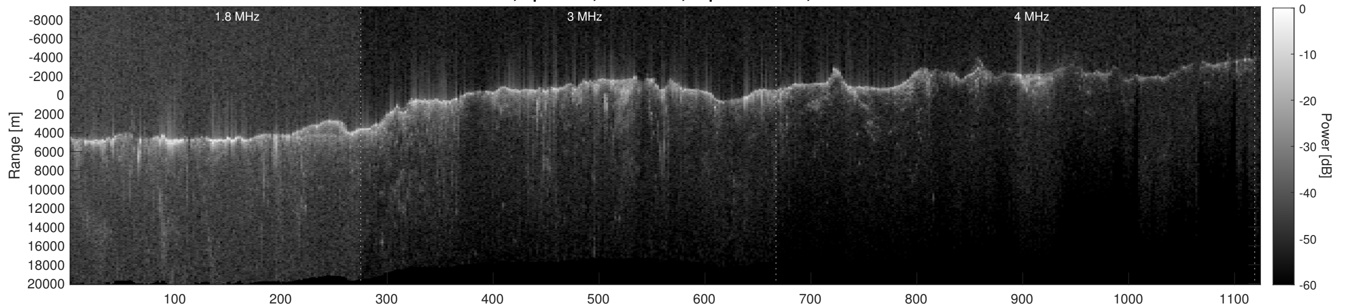
Orbit 7013, Depth-Corrected Cluttergram
