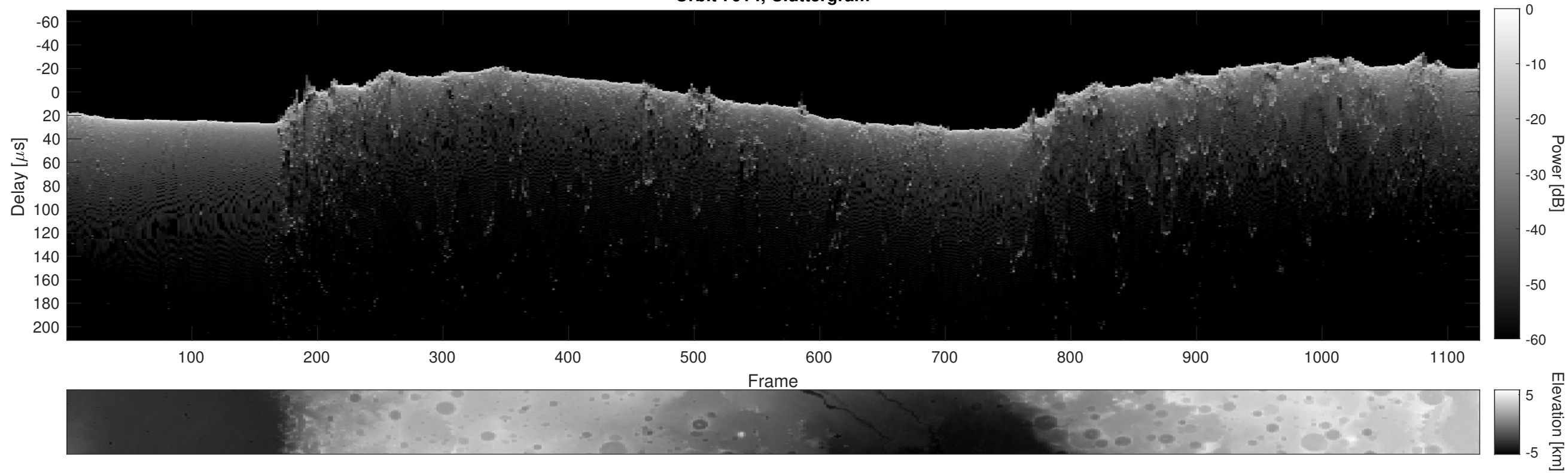
Orbit 7014, Cluttergram
