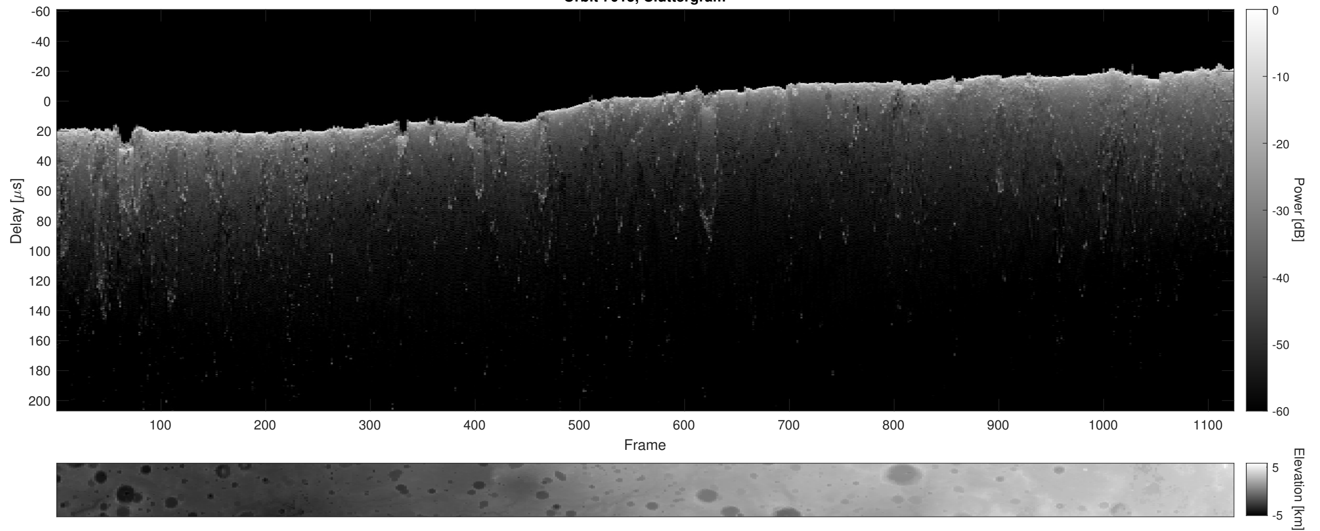
Orbit 7015, Cluttergram
