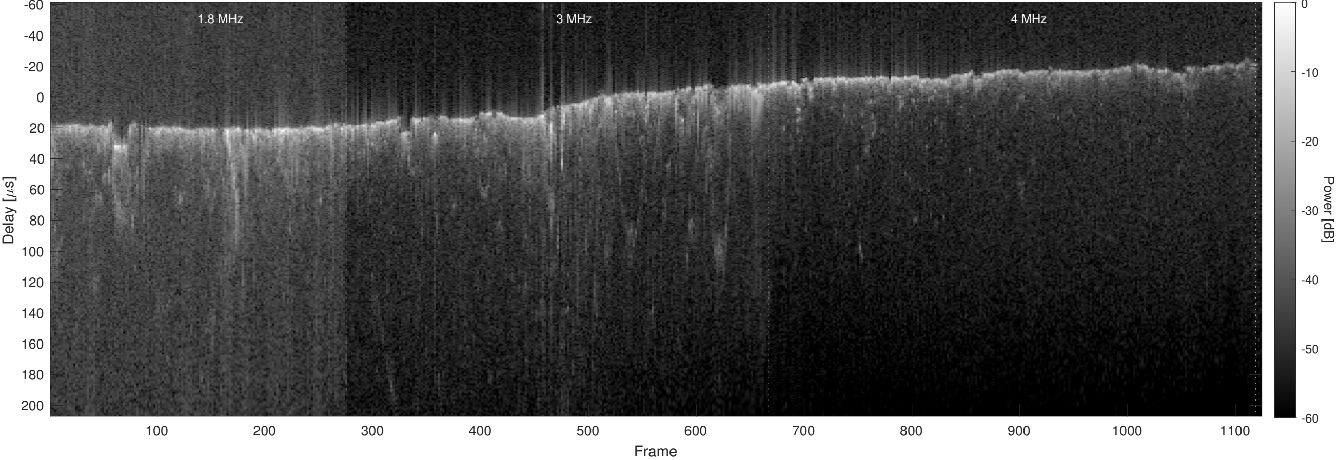
Orbit 7015, Optimized, No Window, Channel 2
