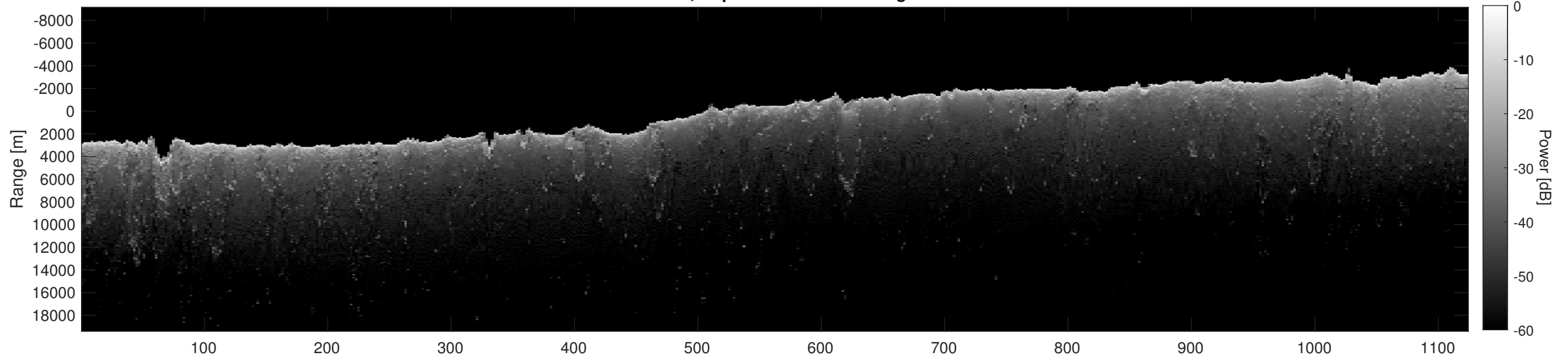
Orbit 7015, Depth-Corrected Cluttergram
