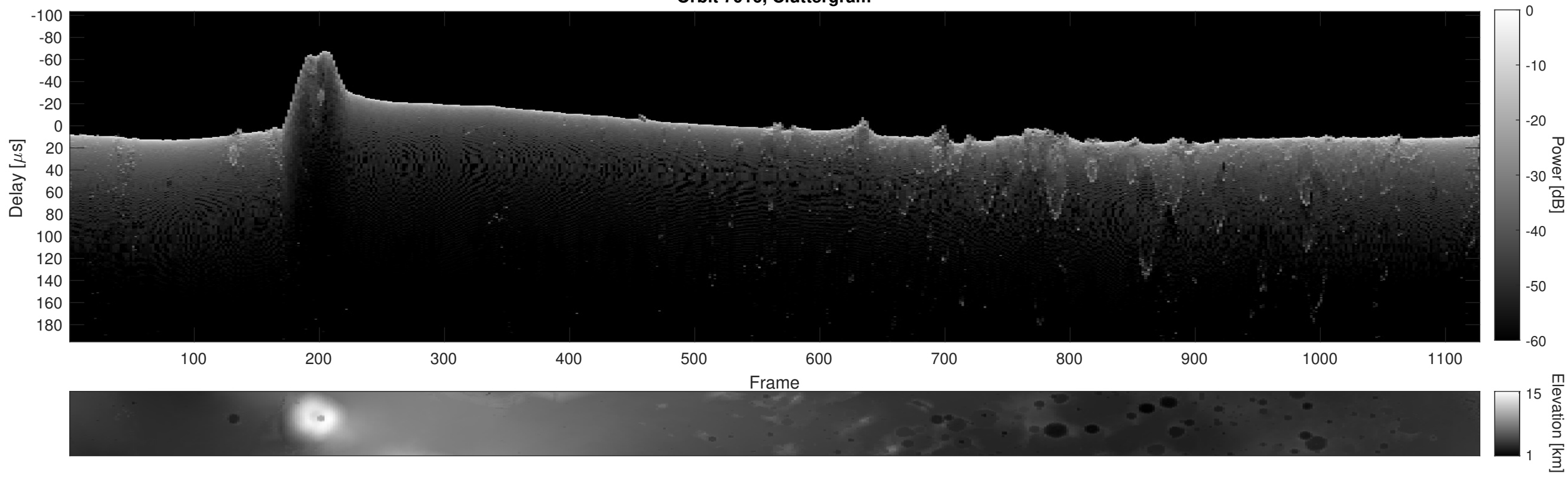
Orbit 7016, Cluttergram
