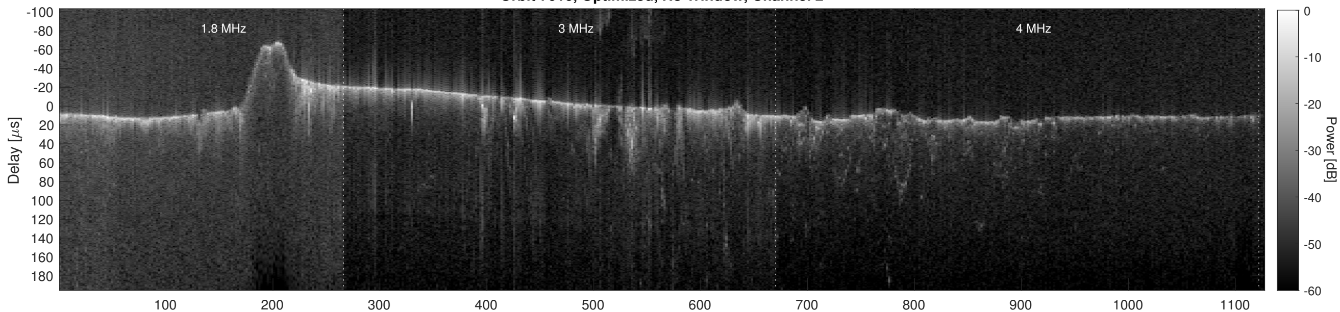
Orbit 7016, Cluttergram
