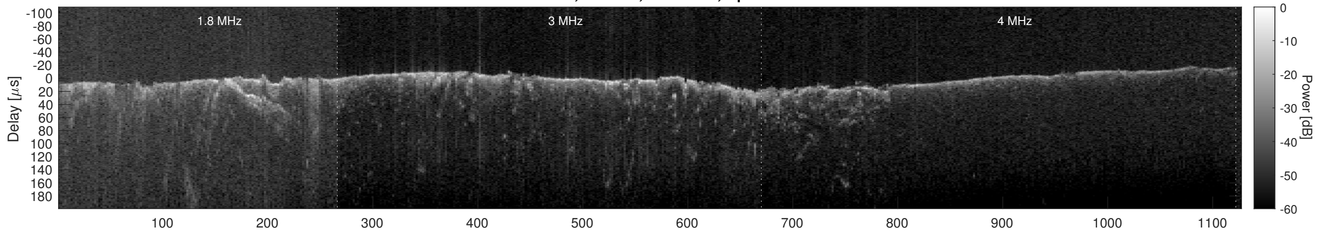
Orbit 7018, Cluttergram
