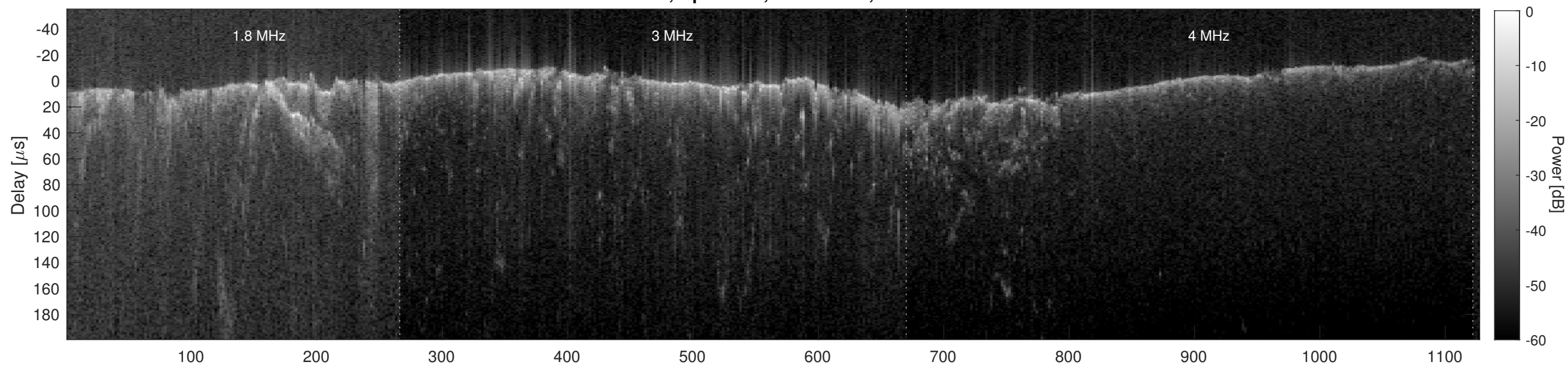
Orbit 7018, Cluttergram
