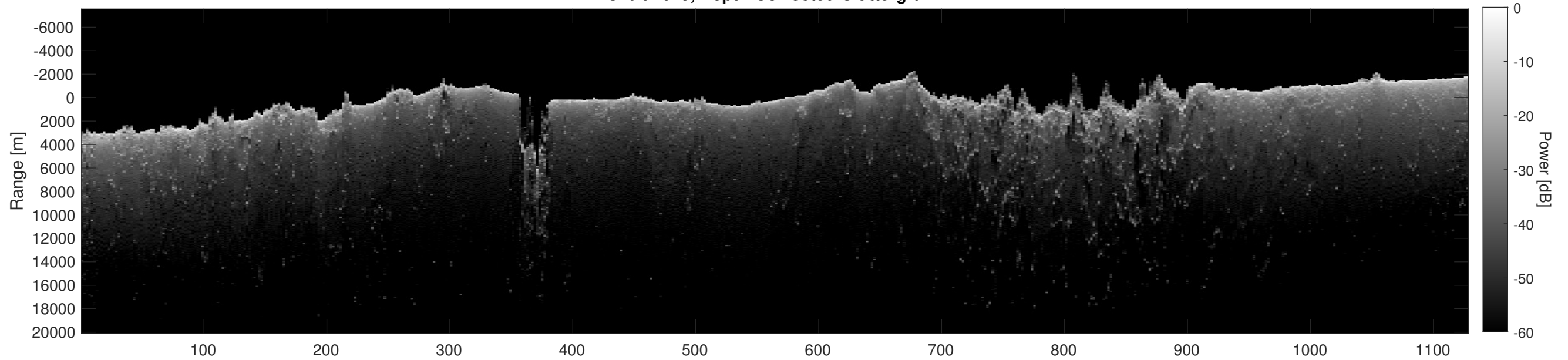
Orbit 7019, Depth-Corrected Cluttergram
