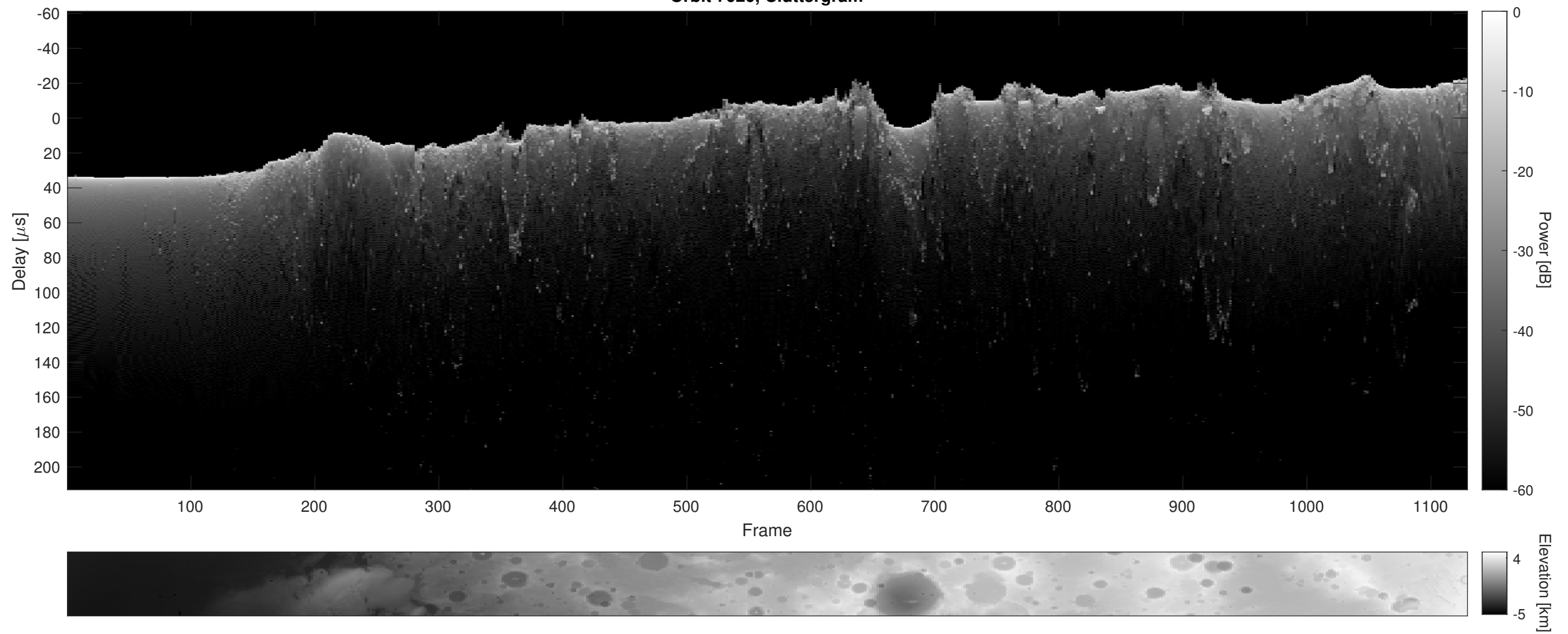
Orbit 7020, Cluttergram
