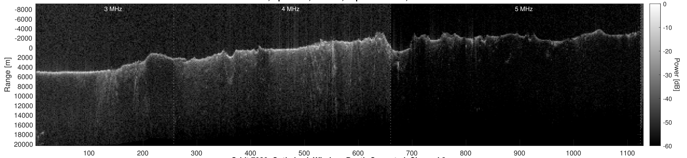
Orbit 7020, Optimized, Window, Depth-Corrected, Channel 2
