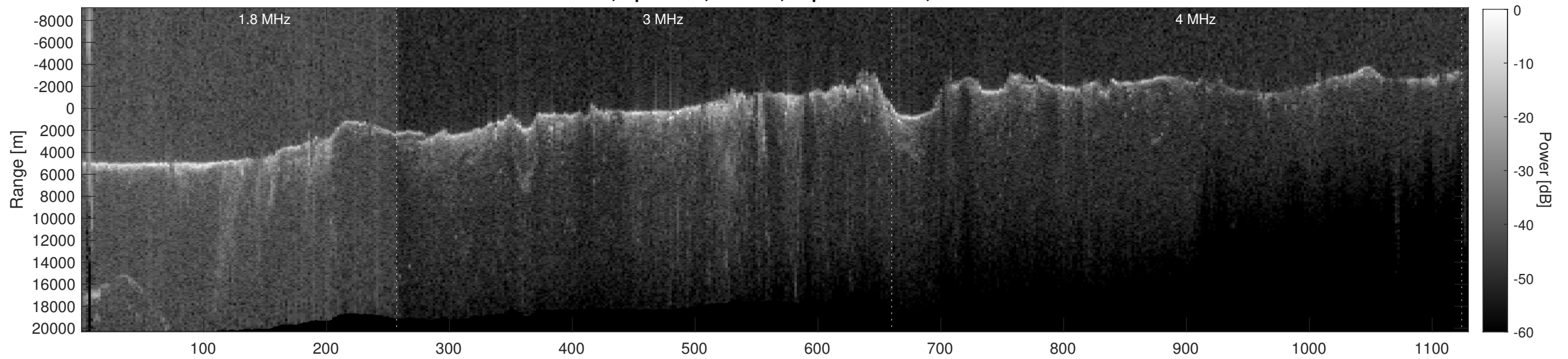
Orbit 7020, Depth-Corrected Cluttergram
