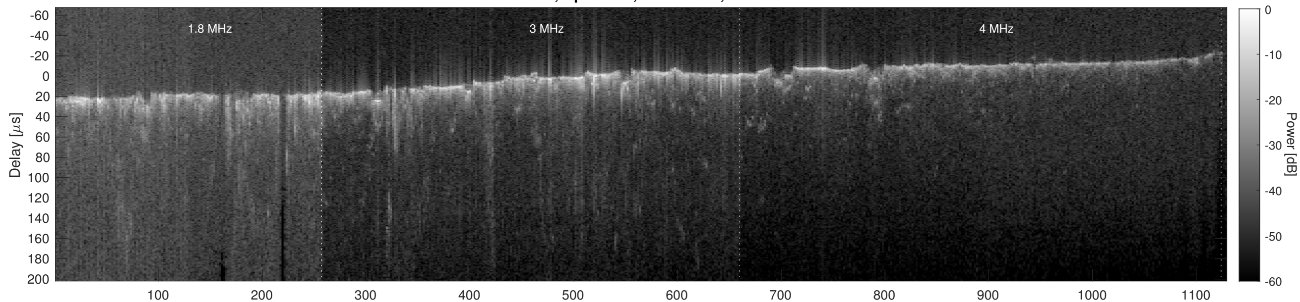
Orbit 7022, Cluttergram
