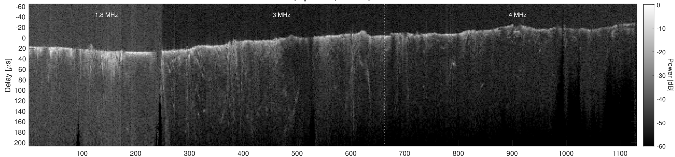
Orbit 7024, Cluttergram
