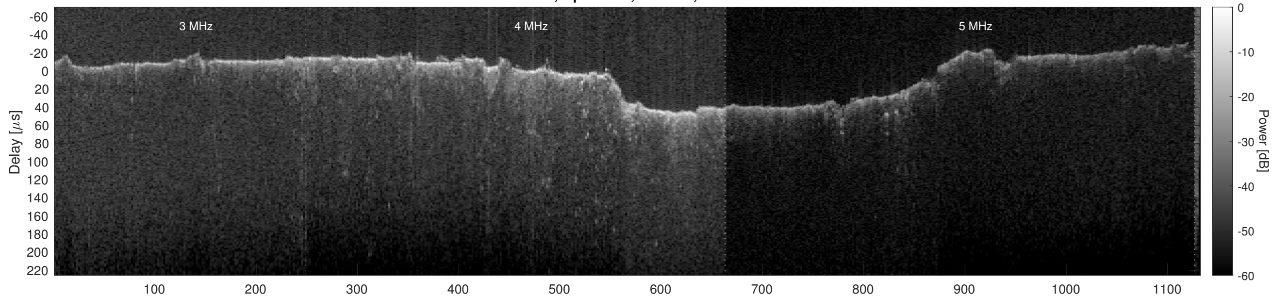
Orbit 7025, Optimized, Window, Channel 2
